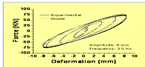
Hysteretic Damper Behavior
